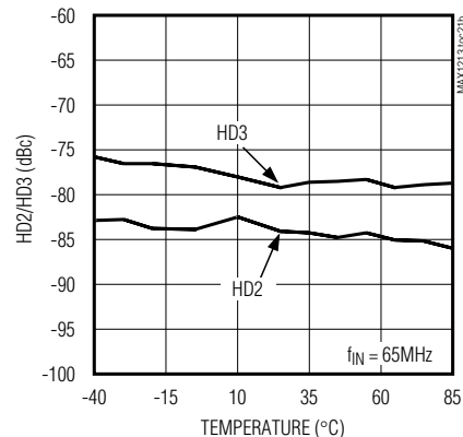
HD2/HD3 vs. TEMPERATURE ( f_{SAMPLE} = 170MHz , A_{IN} = -2dBFS )
