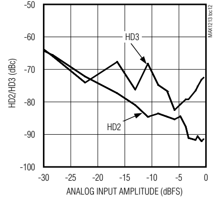
HD2/HD3 vs. ANALOG INPUT AMPLITUDE ( f_{SAMPLE} = 170.0053MHz , f_{IN} = 65.1113MHz )
